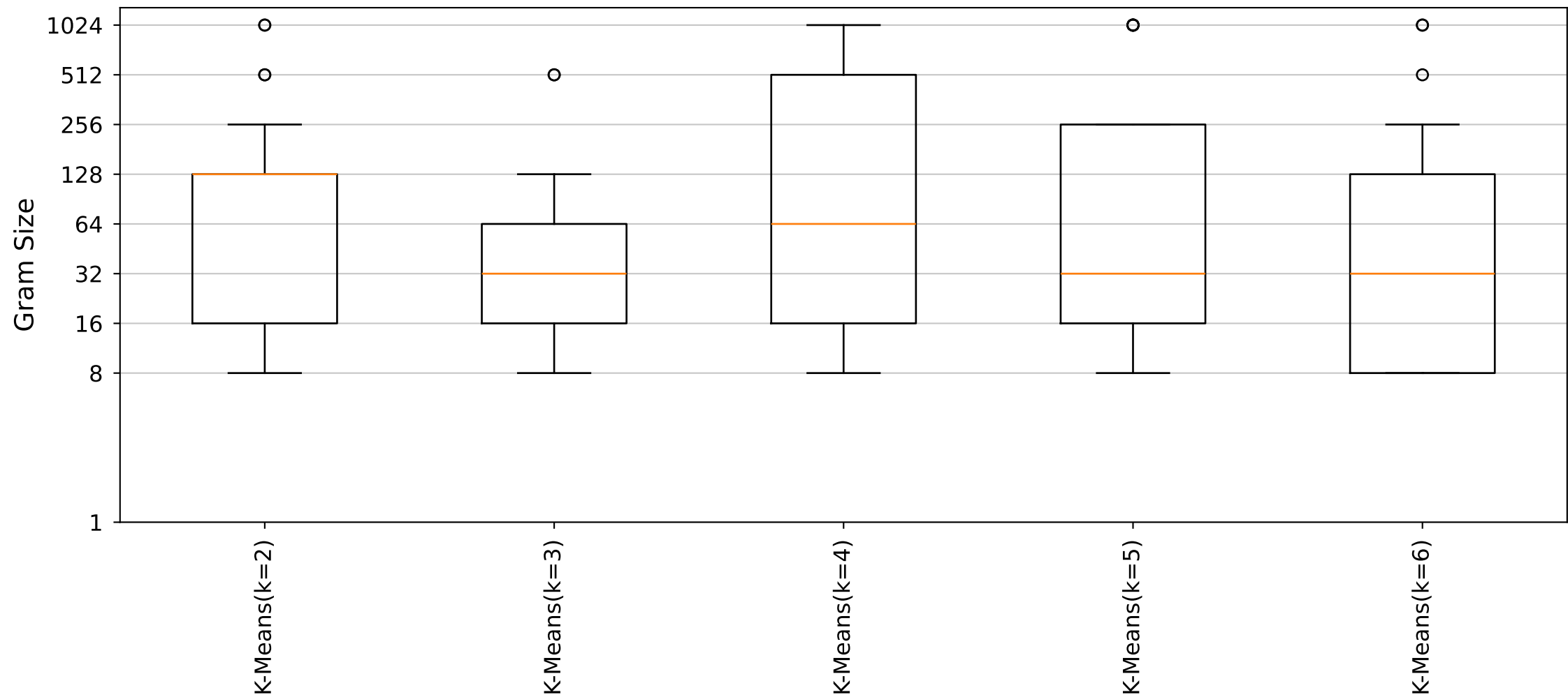
YARA Rules Gram Size Distribution (Cluster19_Size6 dataset)
